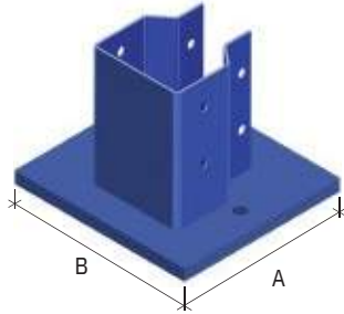
Heavy-Duty Foot Plate UA10
