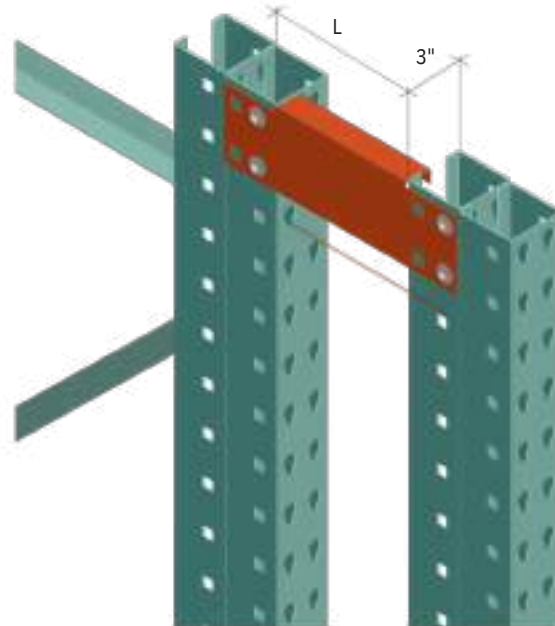
Model 465 in face-to-back arrangement L = Space between posts
