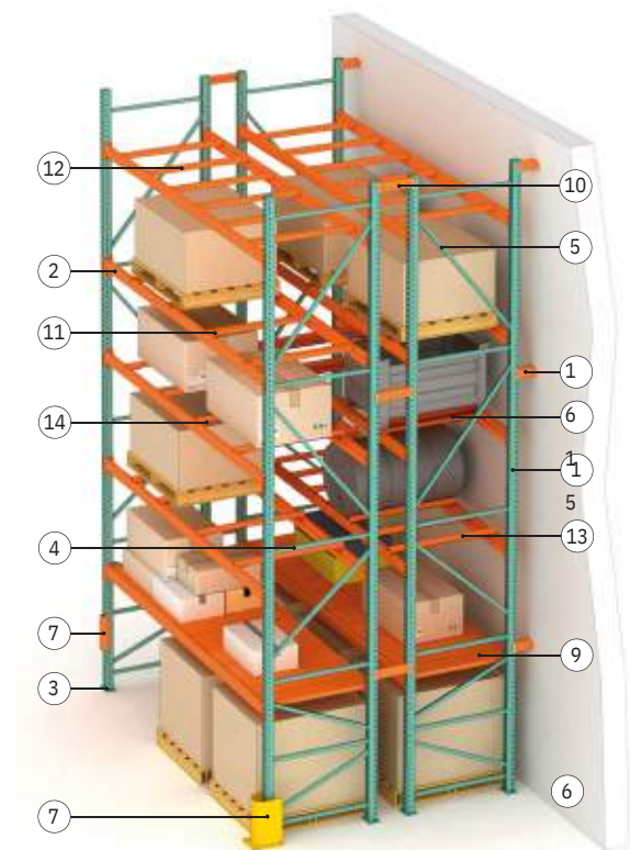
Welded Selective Pallet Rack
