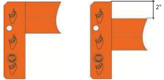
0.00" Beam Drop
