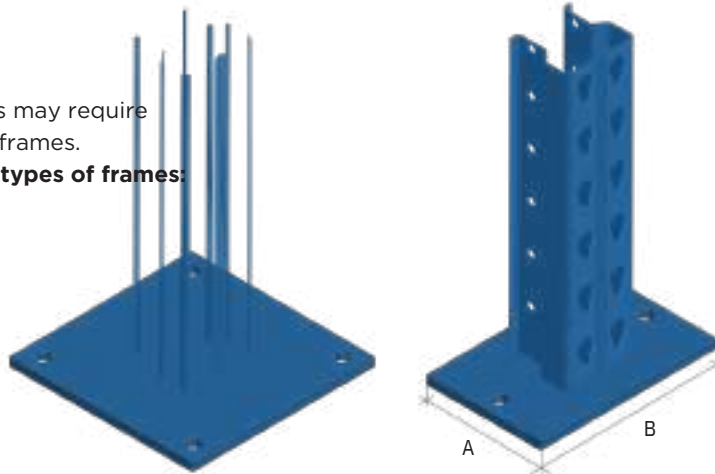
Welded PP Foot Plate
