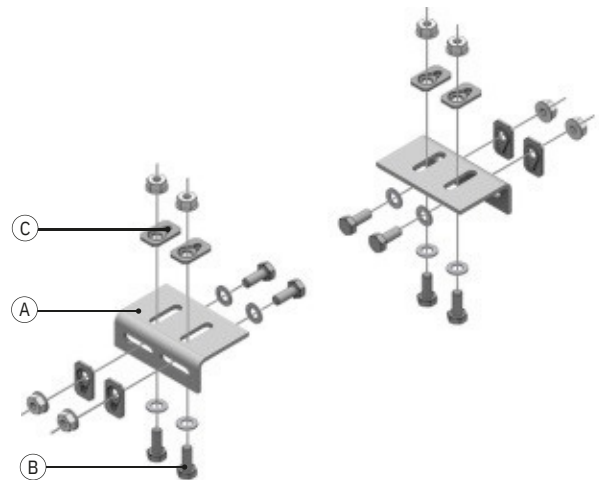
Arm Bracket (T0032605)
